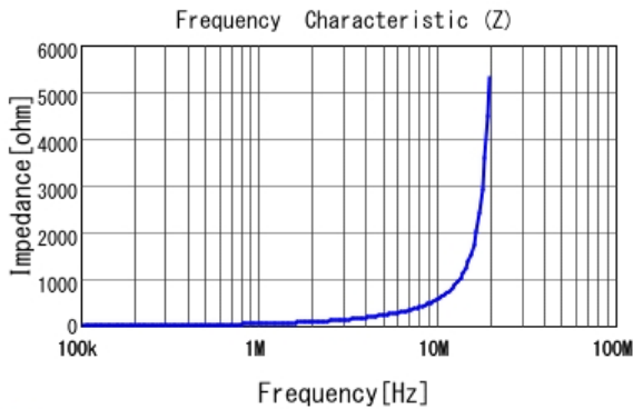
■ 1277AS-H-6R8M |Z|
