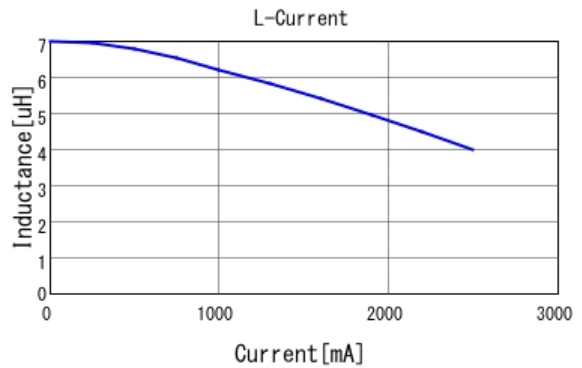
■ 1277AS-H-6R8M L-Current 20degC
