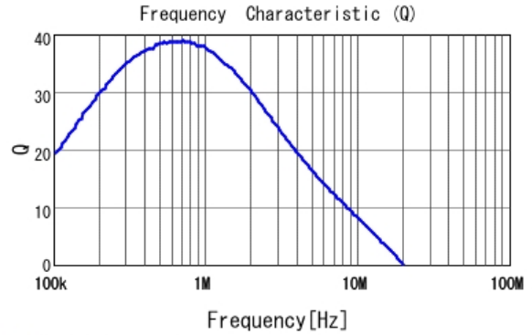
■ 1277AS-H-6R8M Q
