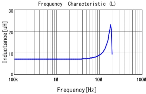
■ 1277AS-H-6R8M L
