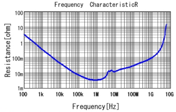
■ GRM21BR6YA106ME43 R DCOV, 25degC
