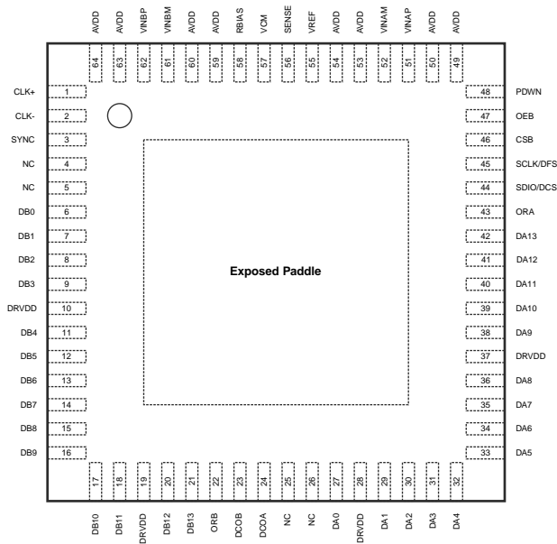
Figure 5: SD9258 Package Top View for Parallel CMOS Configuration.
